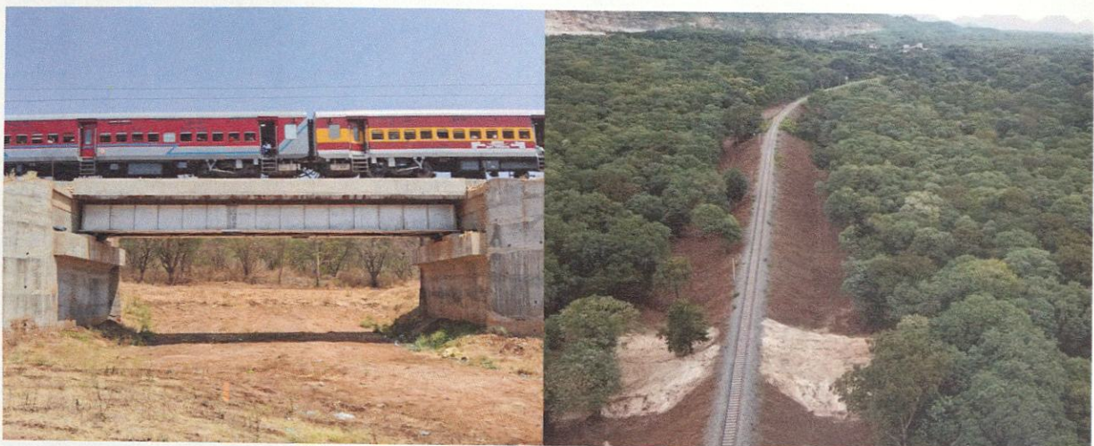
Figure 5: Mitigation structures in Madukkarai Forest range. Left – Underpass of 10 x 18 m dimension; the structure requires installation of light and sound barriers on both sides. Right – level crossing ramp, the structure requires upgradation to make a rubberized level crossing on the track.
