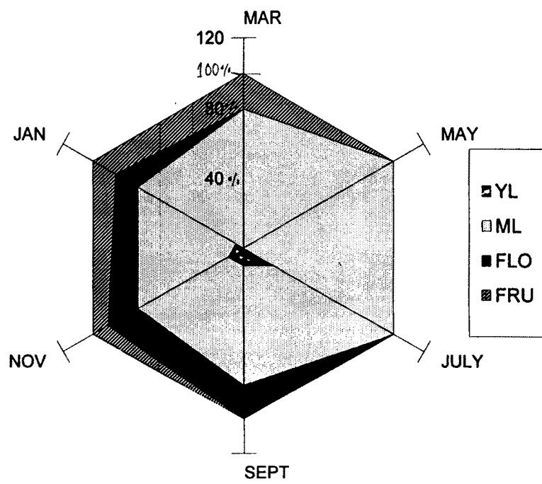
Figure 5.4.6 Phenology of Sida rhombifolia
