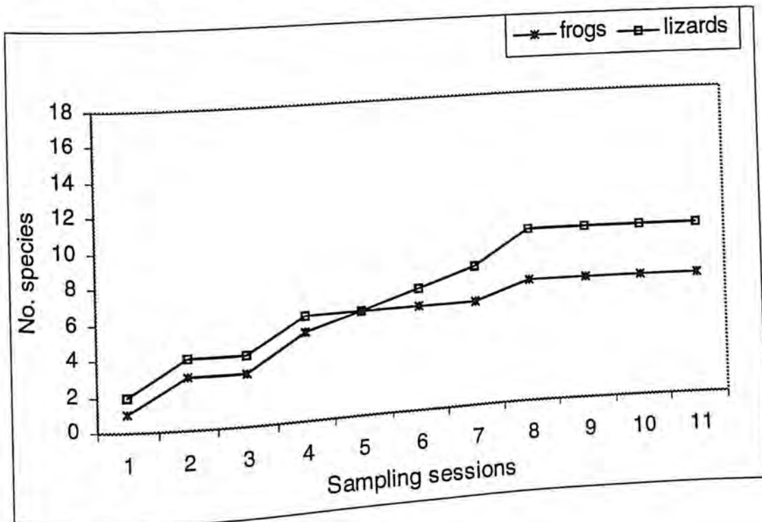
Figure 11: Separate species accumulation curves for frogs and lizards: 30-35yr jhum fallows
