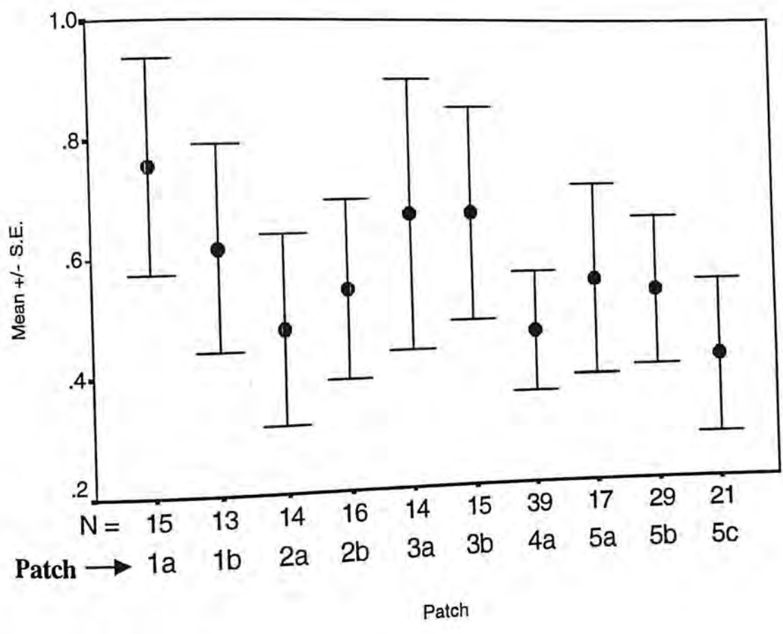
Figure 13: Pooled abundance of frogs and lizards (per 100 m 2 ) across patches (Refer to table 1 for patch label identities)
