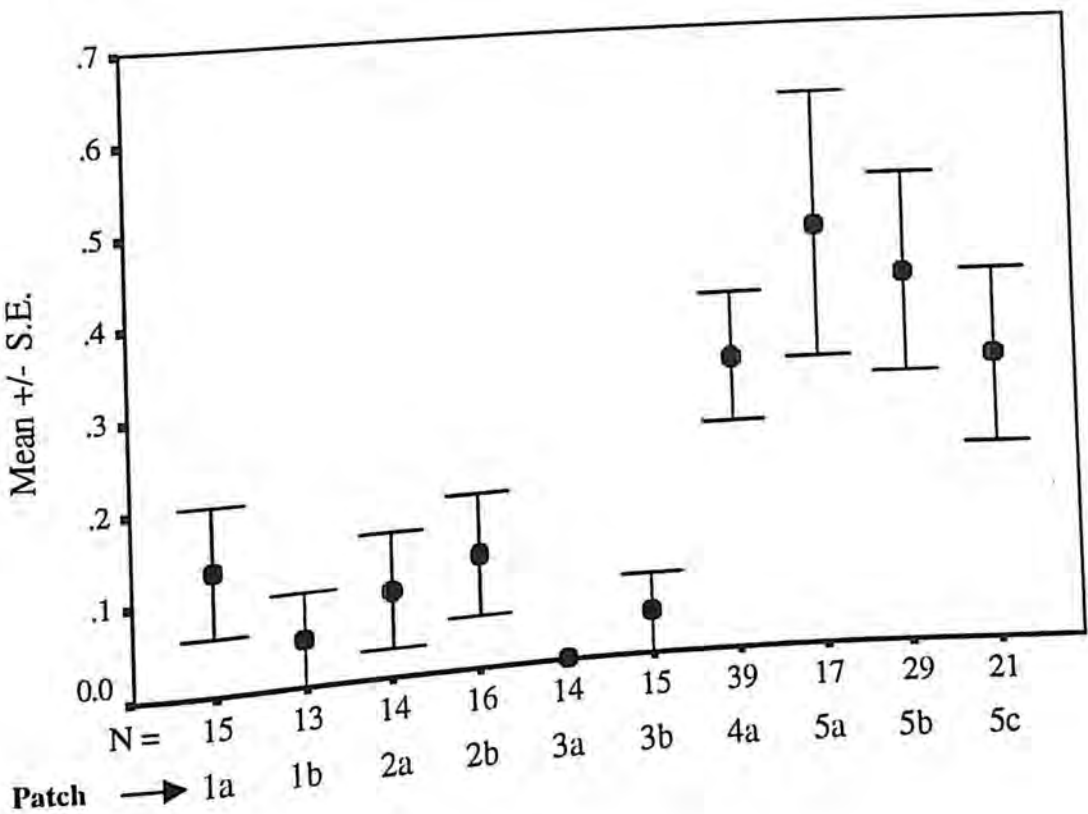
Figure 15: Abundance of nocturnal species (per 100 m 2 ) across patches (Refer to table 1 for patch label identities)
