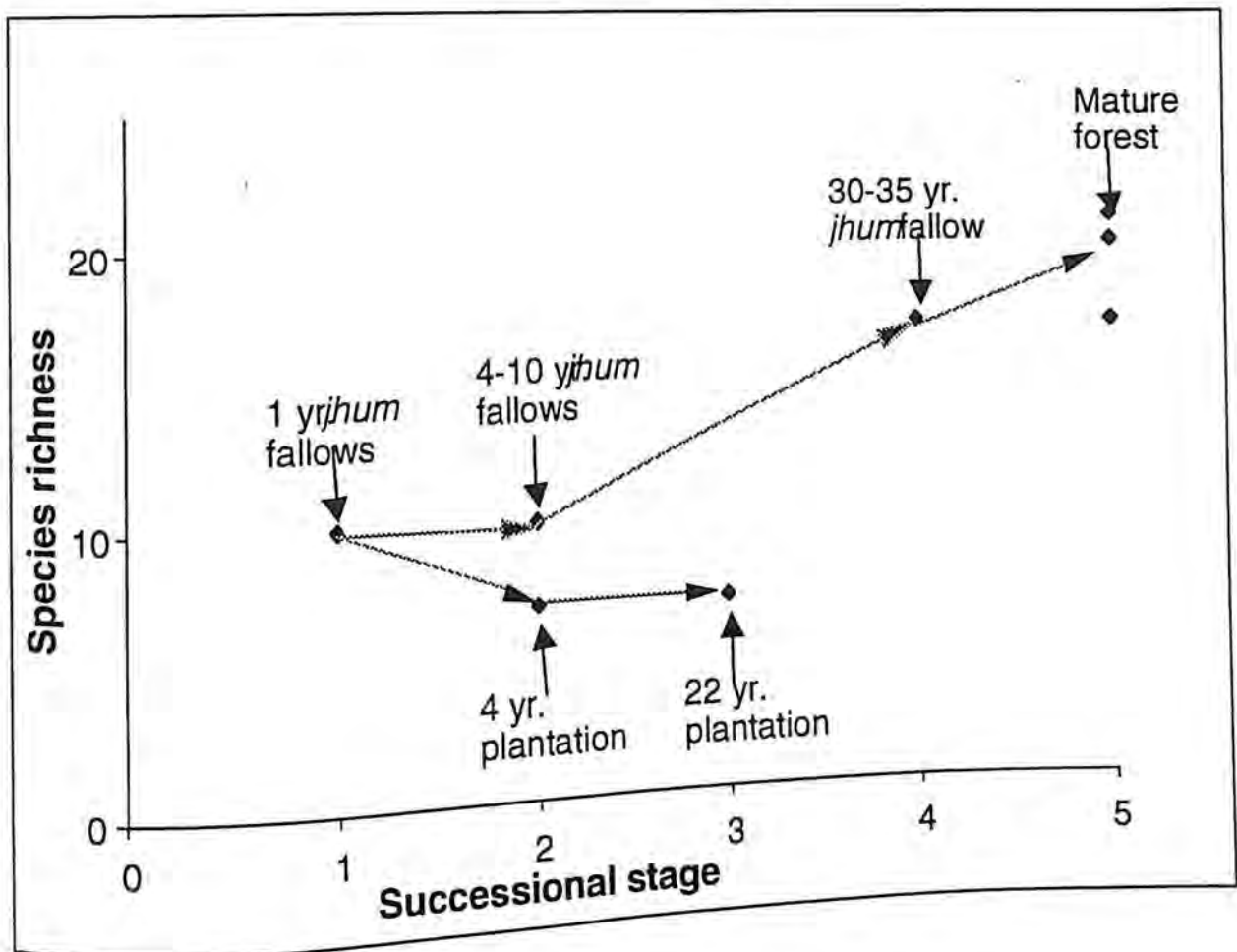
Figure 20: Trends in species richness along successional gradients
