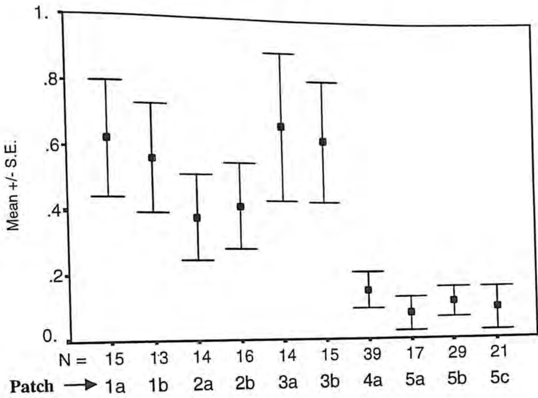
Figure 14: Abundance of diurnal species (per 100 m 2 ) across patches (Refer to table 1 for patch label identities)
