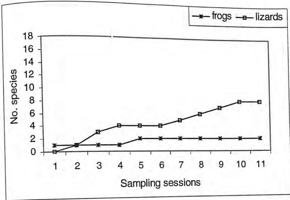
Figure 10: Separate species accumulation curves for frogs and lizards: 4-10yr jhum fallows
