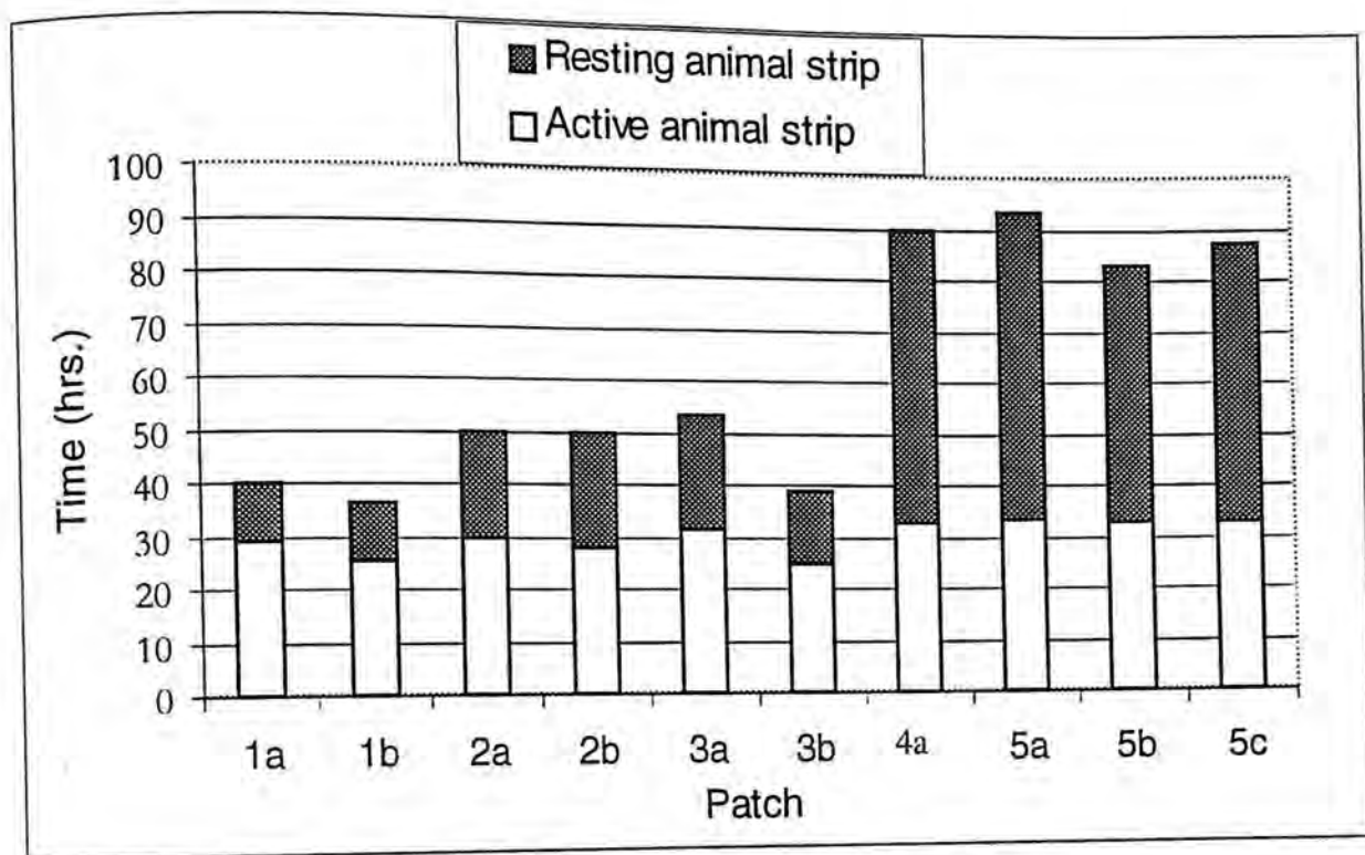
Figure 6: Proportion of sampling time spent on resting and active animal strips across patches
