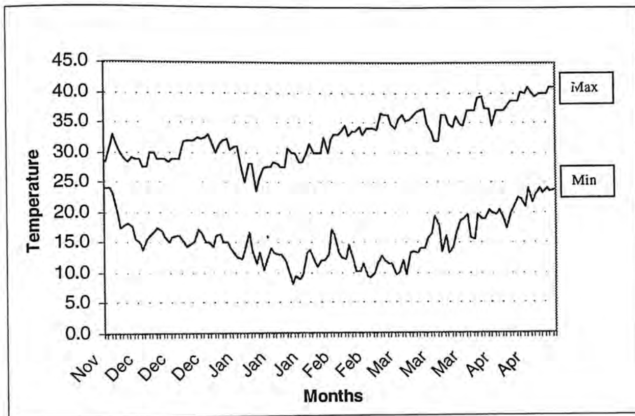
Figure 3: Temperature changes in study area during fieldwork period
