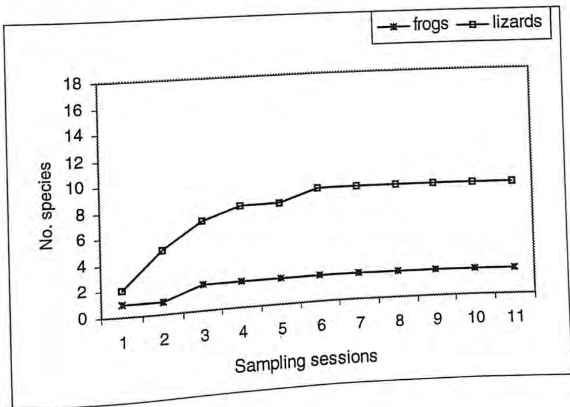
Figure 9: Separate species accumulation curves for frogs and lizards: teak plantations
