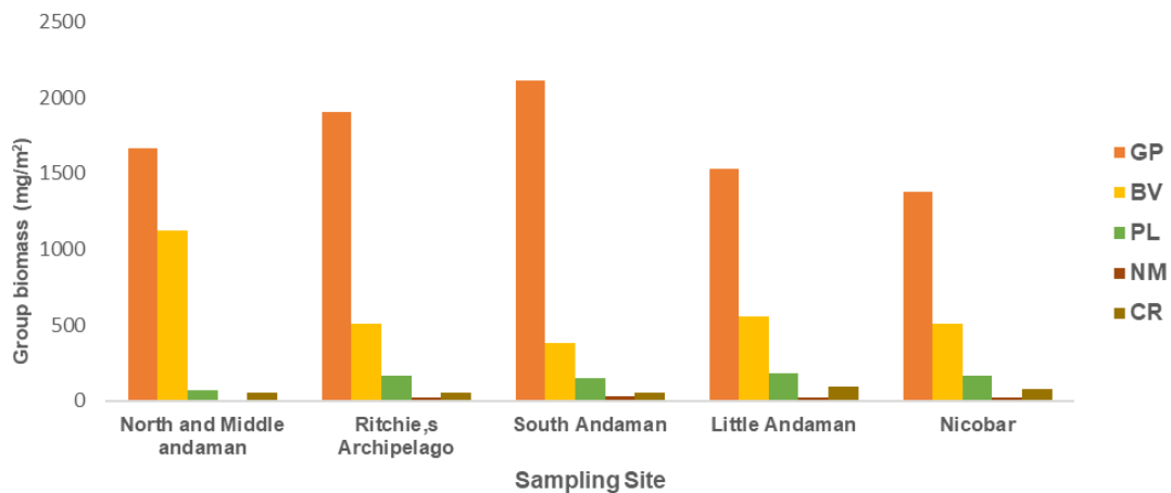
Figure 98. Site-specific biomass of each infaunal groups
