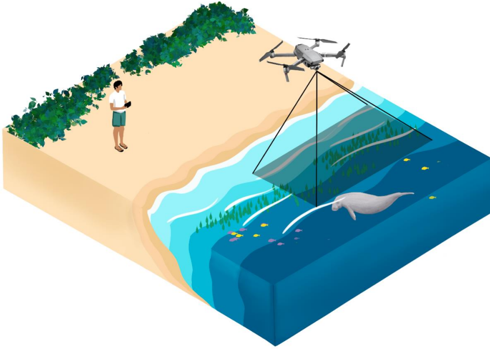
Figure 78. Aerial Survey Study design representation
