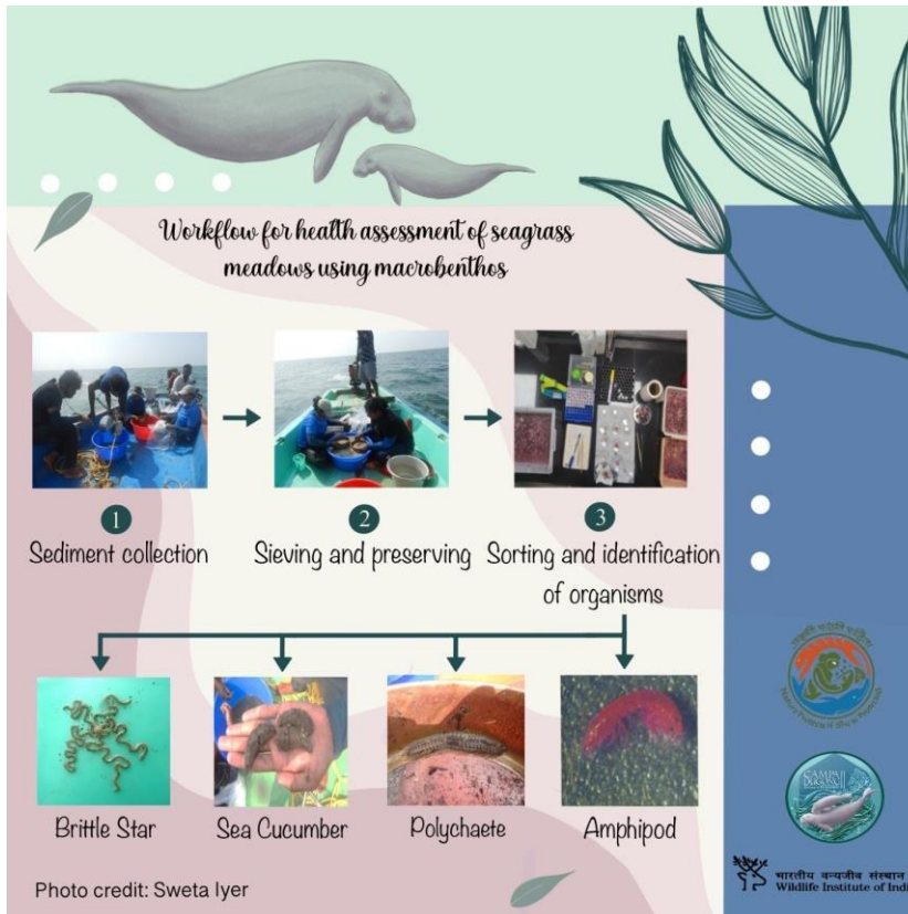
Figure 122. World Dugong Day post Day 12
