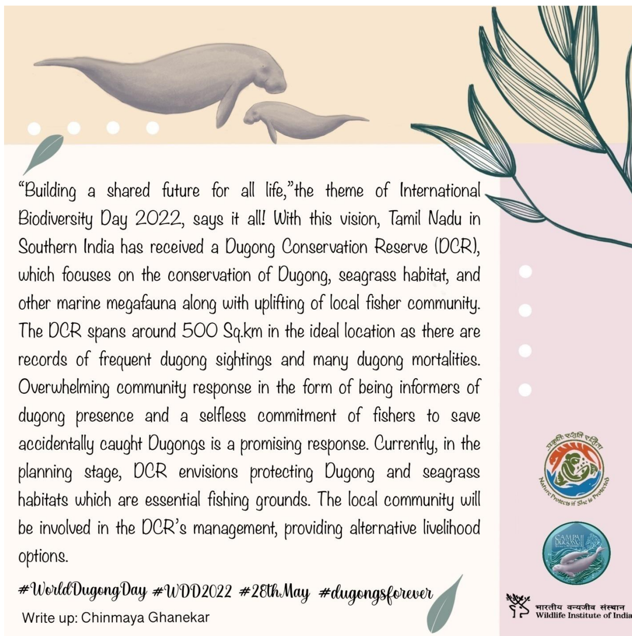
Figure 123. World Dugong Day post Day 14
