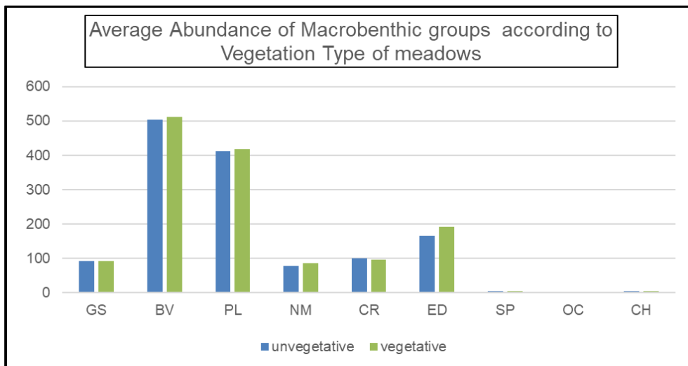
Figure 52. Average Abundance of Macroinvertebrate groups according to Vegetation Type
