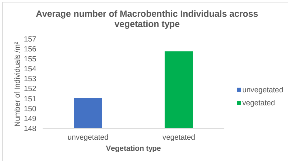
Figure 51. Average number of macroinvertebrate individuals found in respective vegetation type
