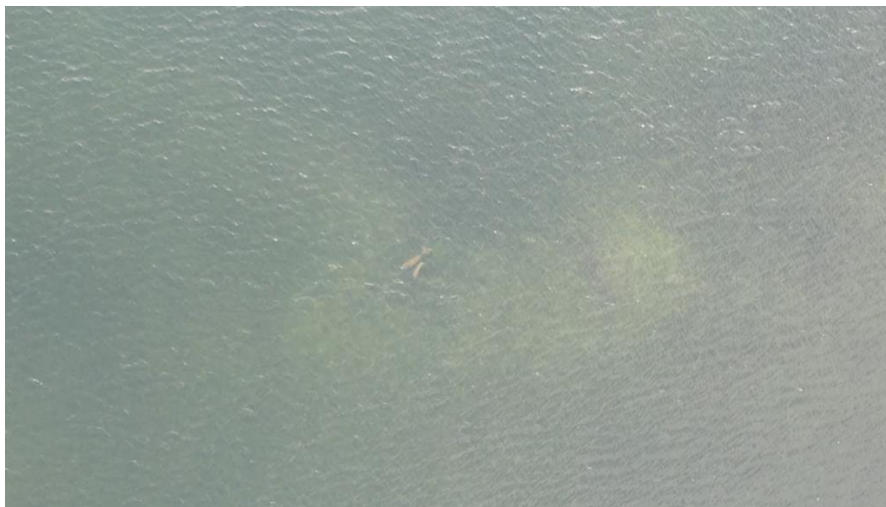
Figure 33. Dugong mother and calf observed at Sethubavachattram.
