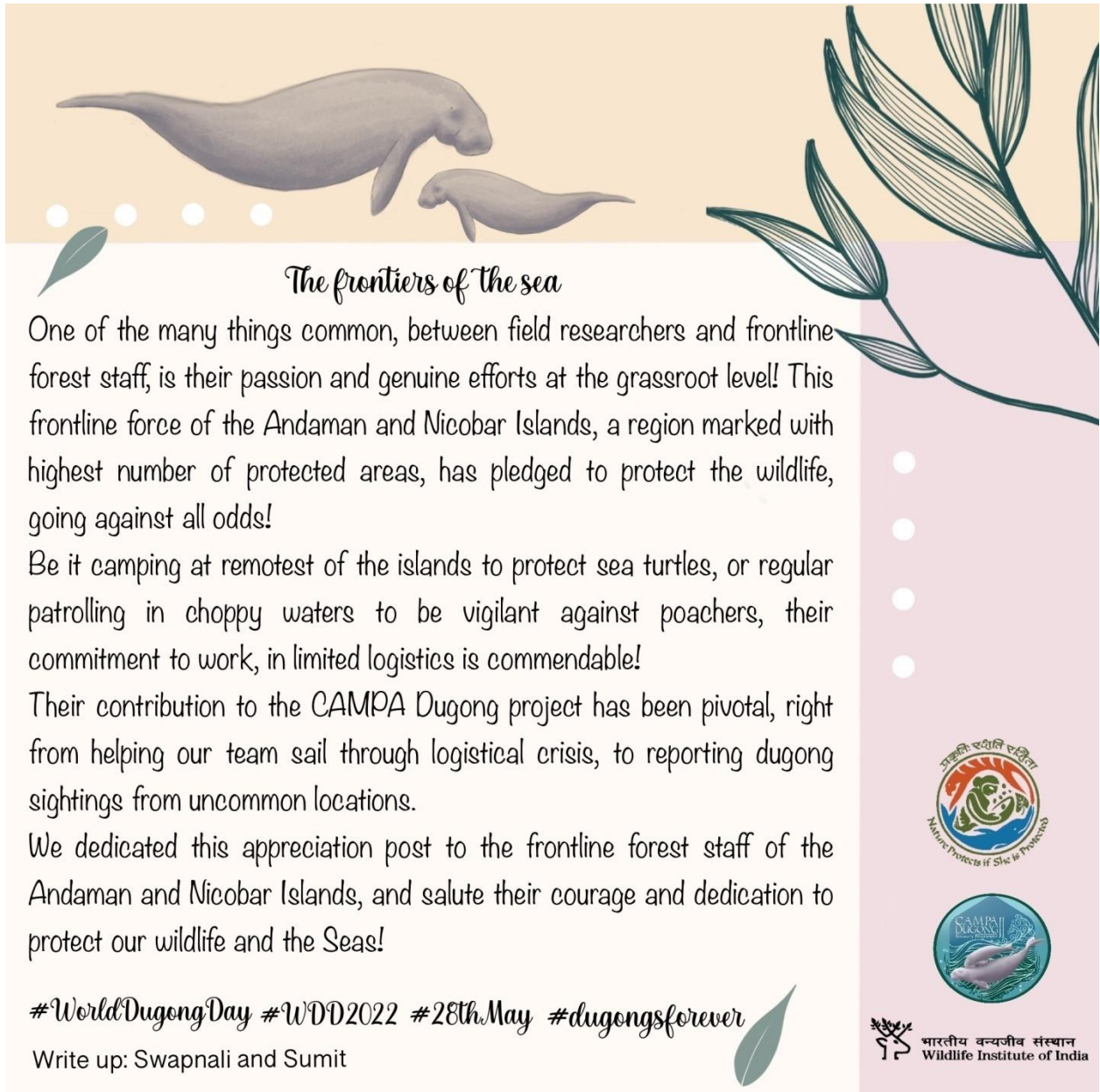
Figure 132. World Dugong Day post-Day 16
