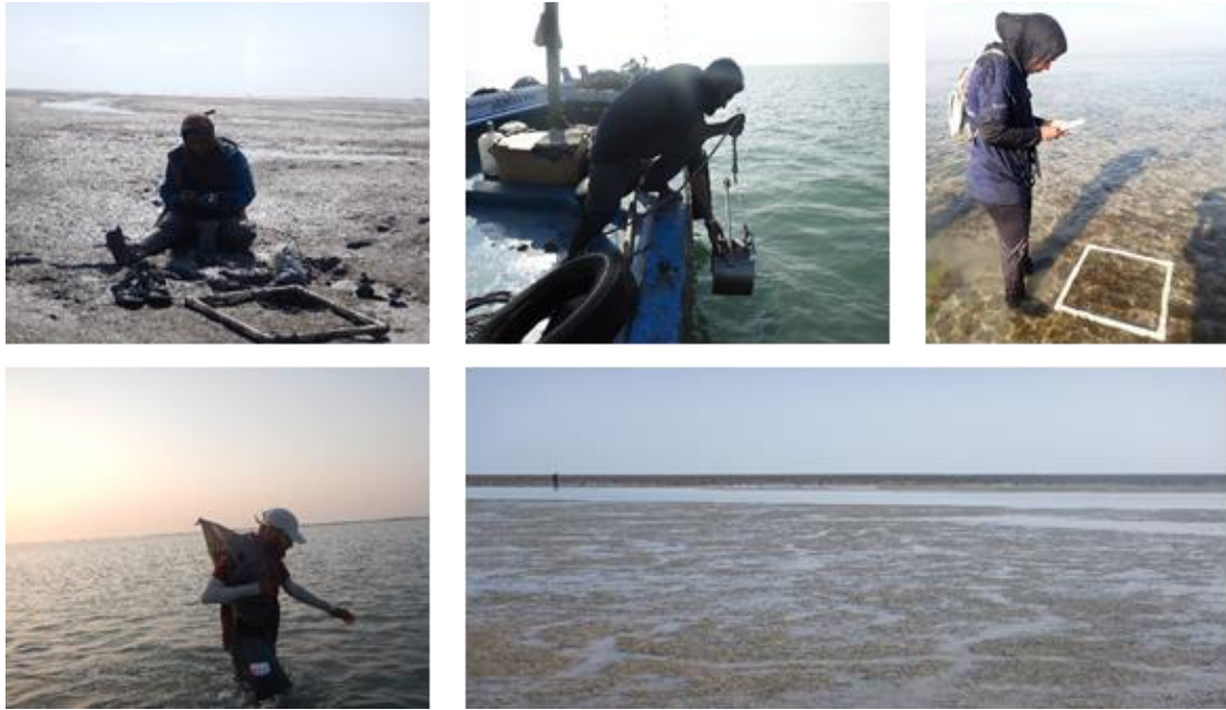
Figure 4. Sampling during the seagrass phenology surveys, Bottom right: Foraging trails were found at Nor reef
