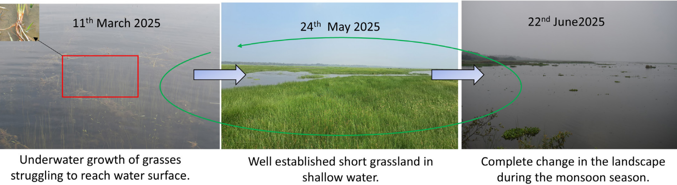
Annual successional dynamics of short grasslands at Haiderpur wetland
